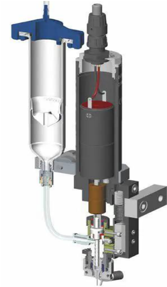
Precision volumetric dispensing with Auger pump (picture: property of NORDSON EFD)
